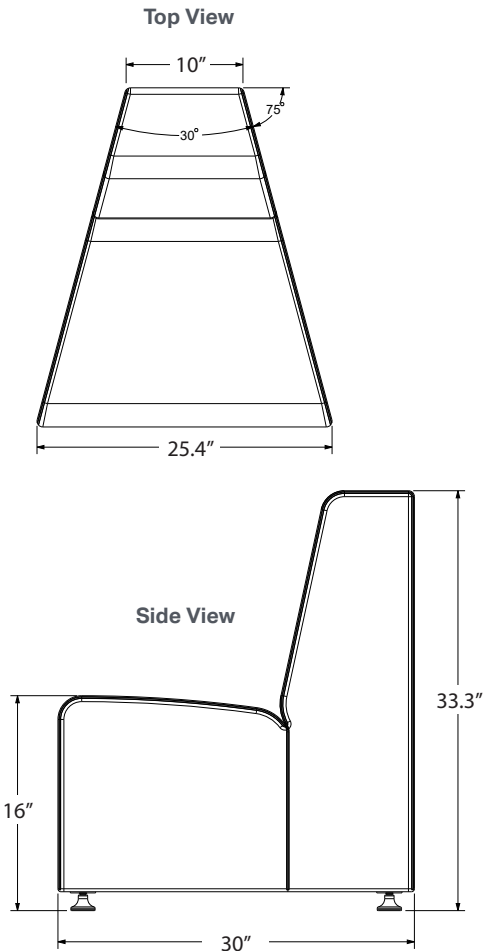
Outer Wedge Chair Model LF1032
