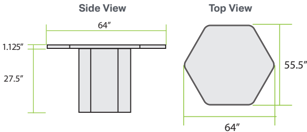
Hexagon Table Model LF2653
