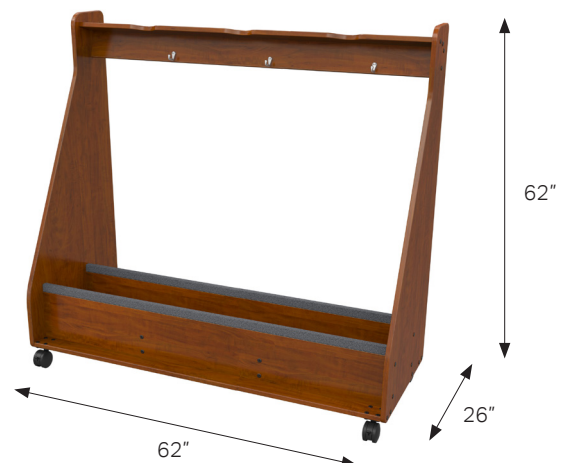
BS501 String Bass Rack (3 units)
