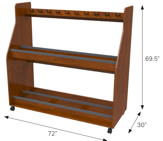
BS500 Guitar Rack
